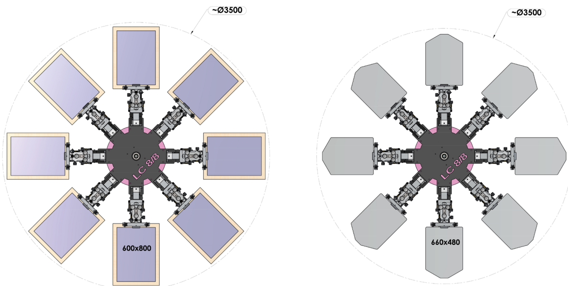
Dimensional drawing - 8 posts
